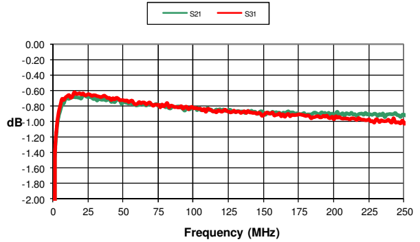
Insertion Loss
